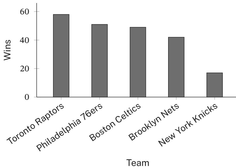
Figure 17. Ordering by wins clarifies the ranking, but the rotated names are still read at an angle.
