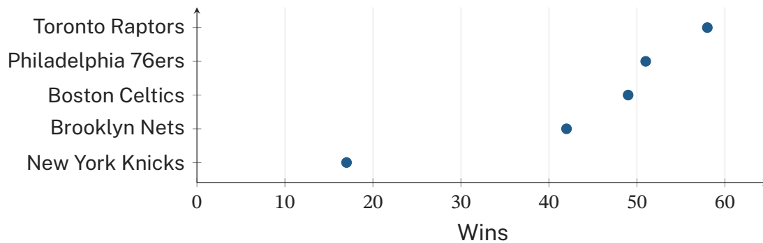
Figure 19. The same five 2018–19 amounts represented by positions.
