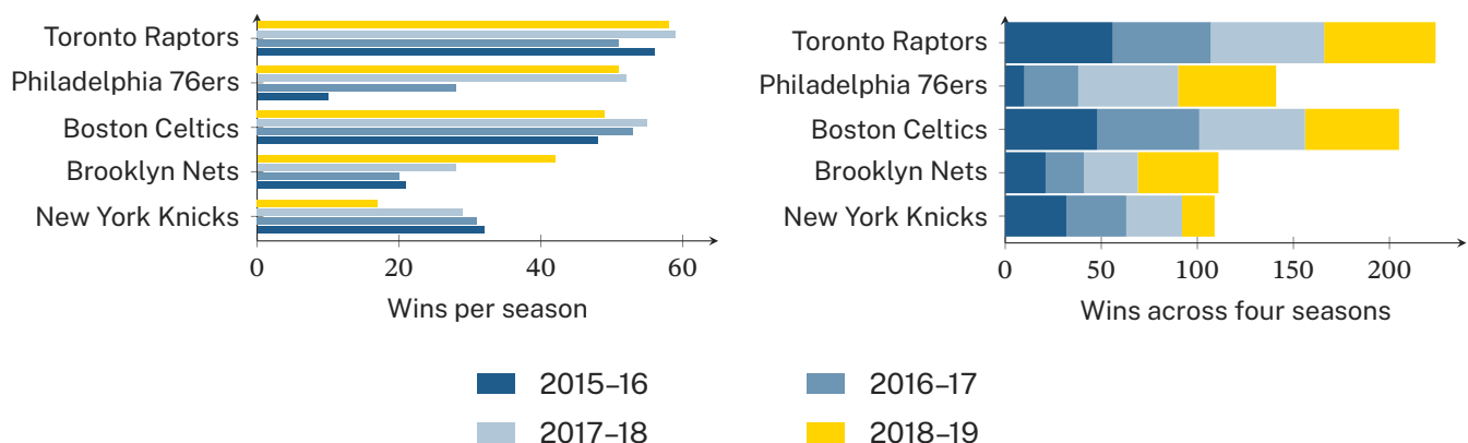
Figure 20. The same twenty values in grouped and stacked form. Seasons run 2015–16 to 2018–19, bottom to top within groups and left to right within stacks. Position also identifies each season when colours are difficult to distinguish.
