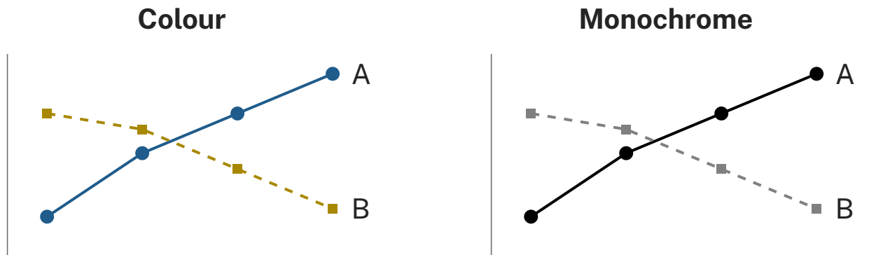
Figure 15. The labelled groups remain distinguishable in colour and monochrome. This comparison is not a physiological simulation of any particular colour-vision condition.
