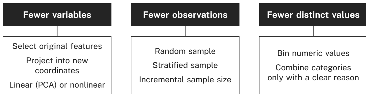
Figure 1. Three ways to simplify a table. Resampling is a broader family of methods; it does not always reduce the number of rows.
