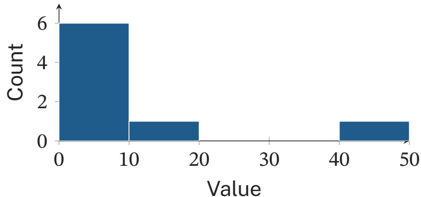
Figure 11. A single fixed dataset and bin specification gives the same counts in both languages.
