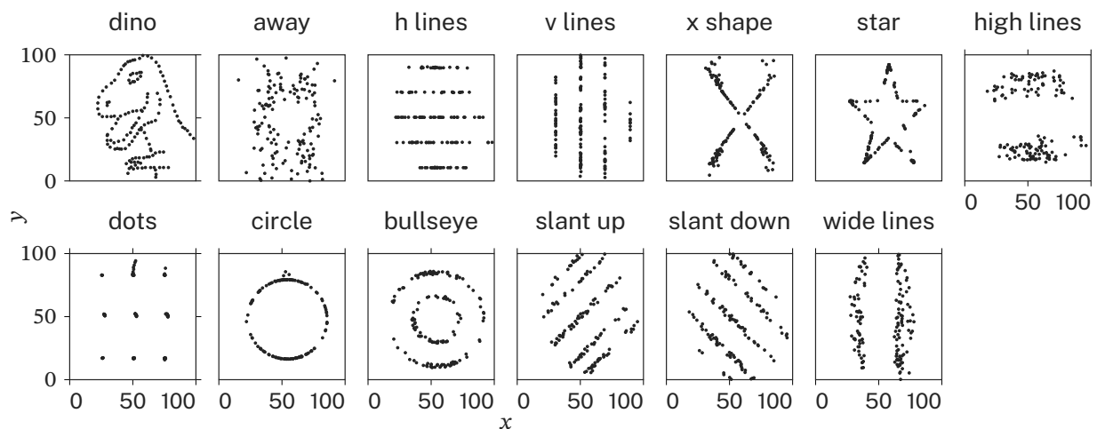
Figure 8. The authentic thirteen datasets. All panels use 0–100 on both axes. Each panel has 142 points.
