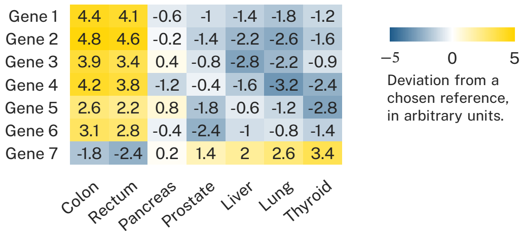
Figure 21. A matrix with an explicit reference. Blue represents negative deviations, white represents zero, and gold represents positive deviations. Layout after the Wikimedia Commons example RNA-seq heatmap [2].
