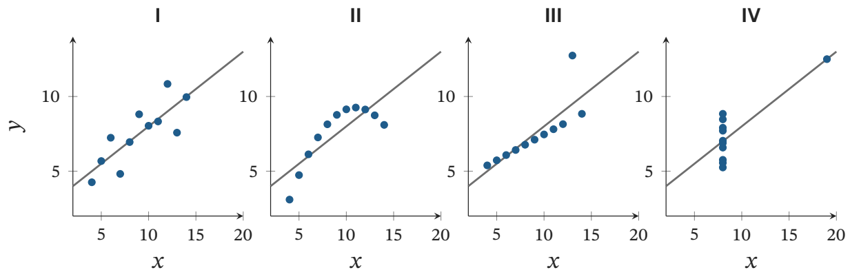
Figure 7. The original quartet on common axes. The grey line is y = 3 + 0.5x , a rounded common fitted line shown for comparison. The task is to inspect the points, not to fit a model.
