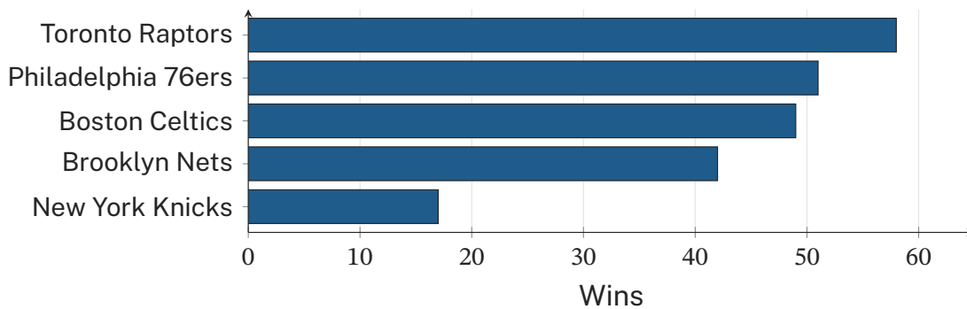
Figure 18. Readable names and a deliberate ranking on the same zero-based scale.
