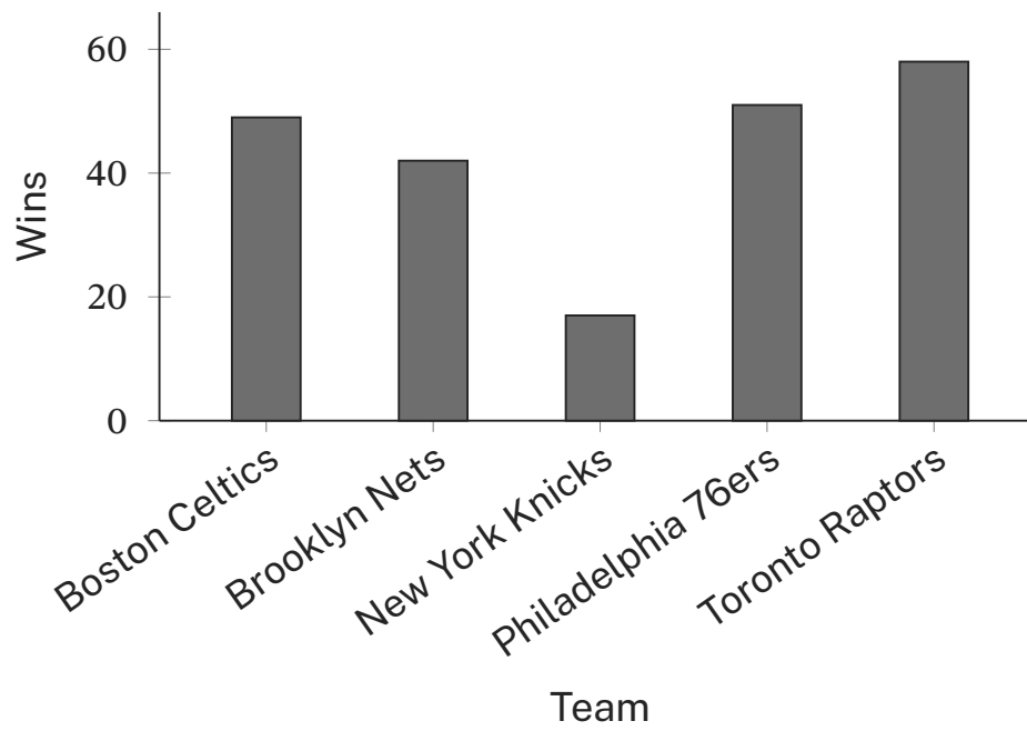
Figure 16. Alphabetical order supports lookup. The long names fit only because they are rotated.
