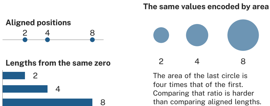
Figure 14. The same three values shown through position, length, and area. Aligned positions make the ratio between the values easier to compare.
